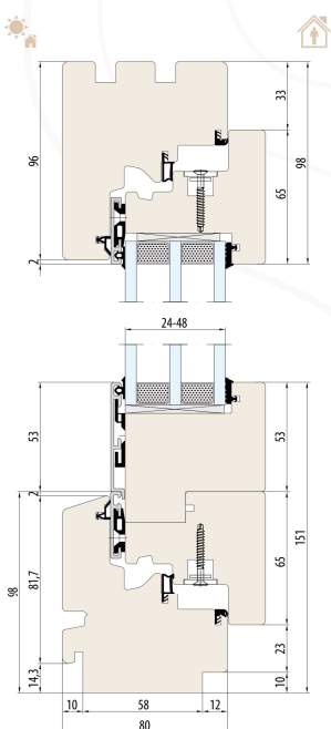
ESPERIA LIFE 80 SYSTEM one-sash balcony doors on high threshold
