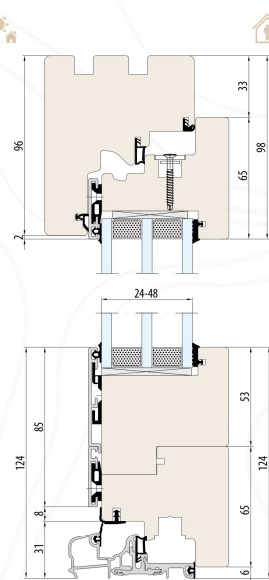
ESPERIA LIFE 80 SYSTEM one-sash balcony doors on low threshold
