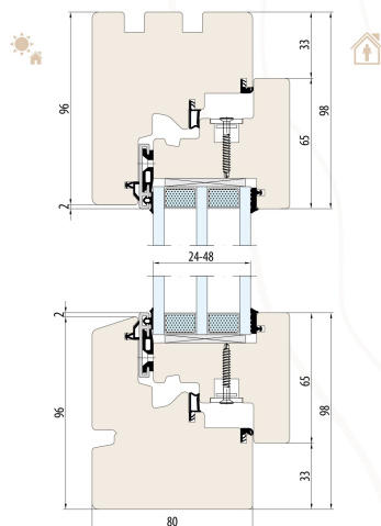
ESPERIA LIFE 80 SYSTEM Without undercut for the window sill
